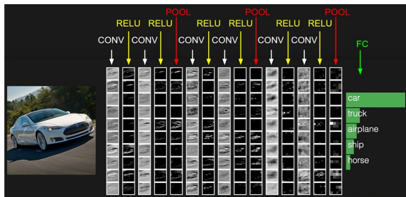
Fig: An example architecture: ([Input] → CONV(ReLU) → CONV(ReLU) → Pool → CONV(ReLU) → CONV(ReLU) → Pool → CONV(ReLU) → CONV(ReLU) → Pool → Flatten → FCN → [Class Scores])
